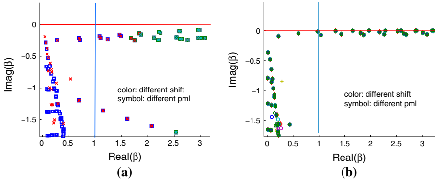
Fig. 5 Numerically computed open resonances found by an Arnoldi algorithm implemented in the hp finite element code NGSOLVE [2]. The different symbols stand for complex eigenvalues of (6.1), see [15] for more detailed explanations. a Non-resonant situation, b near resonance situation (color figure online)
