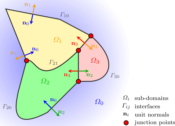
Fig. 1 Typical geometry of a composite scatterer for N = 3 (color figure online)
