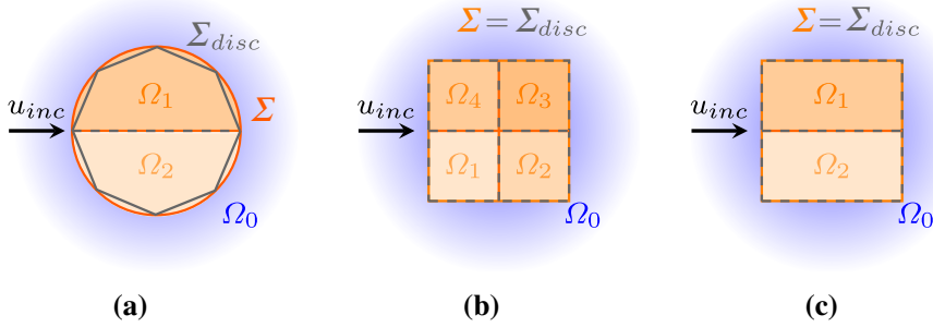
Fig. 3 Geometries for numerical experiments. a Two half discs of radius r = 0.4 , b four quarts of a square of side length s = 0.5 , c two halves of a square of side length s = 0.5 (color figure online)
