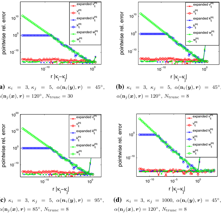
Fig. 2 Convergence of series expansions: depicted are the relative pointwise errors as a function of r|\kappa_i - \kappa_j| , where r := |\mathbf{x} - \mathbf{y}| , of the expansions found in the proof of Lemma 5.3, truncated at N_{\text{trunc}} . The reference solutions are calculated with MATHEMATICA with very high precision, while the other calculations are done in MATLAB. \alpha(\mathbf{n}_i(\mathbf{y}), \mathbf{r}) denotes the angle between \mathbf{n}_i(\mathbf{y}) and \mathbf{r} := \mathbf{x} - \mathbf{y} (color figure online)
