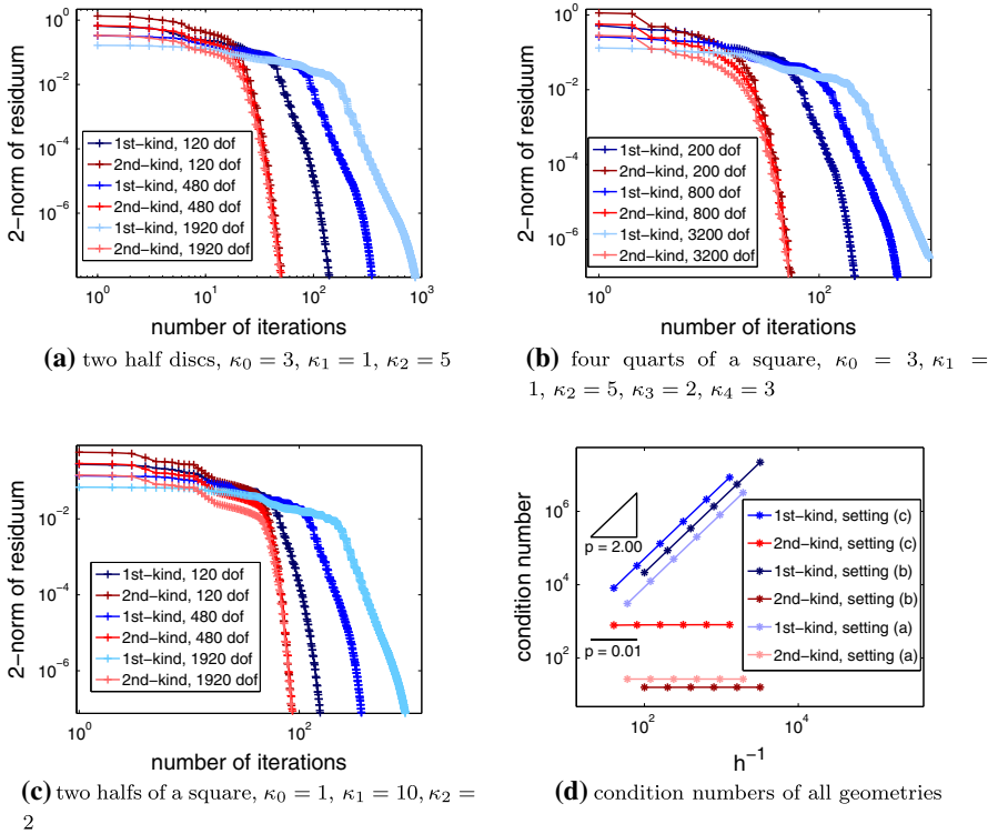
Fig. 7 Euclidean condition numbers of Galerkin matrices with respect to h_{\mathcal{T}}^{-1} and performance of GMRES on Galerkin matrices for different numbers of degrees of freedom (dof, highlighted by different colors). Initial guess used for GMRES is x_0 = \mathbf{0} . The expression “setting (a)” (resp. (b) or (c)) in subfigure (d) refers to the geometric setting given in the particular subfigure (a) (resp. (b) or (c)) of Fig. 3 (color figure online)
