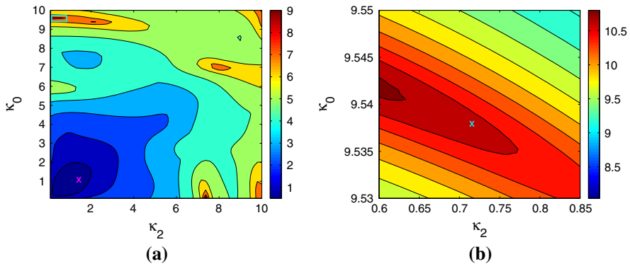
Fig. 4 (Logarithms of) Euclidean condition numbers of Galerkin matrix for various wave numbers: The Galerkin matrix of the second-kind formulation for the situation of two half discs (Fig. 3a) with equidistant mesh, |T| = 480 , is used. The wave number \kappa_1 = 1 is fixed, while \kappa_0, \kappa_2 \in (0.1 : \frac{99}{500} : 10) (for a ) resp. \kappa_0 \in (9.53 : \frac{1}{100} : 9.55) , \kappa_2 \in (0.6 : \frac{35}{200} : 0.85) (for b ). a Global situation, b zoom into area marked by cyan rectangle in the upper left of a (color figure online)
