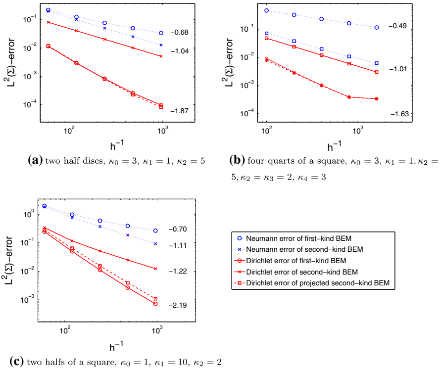
Fig. 6 Convergence in L^2(\Sigma) -norm on equidistant meshes with \frac{3}{2}5 \cdot 2^i cells (scatterer composed of two materials) resp. \frac{5}{2}5 \cdot 2^i , i = 3, 4, \dots, 8 elements (four materials, see Fig. 3 for geometries). The error norms for the Dirichlet and Neumann data are plotted in red and blue, respectively. The graphs show the errors with respect to the solutions calculated with CONCEPTS. They are annotated by estimated rates of convergence (color figure online)
