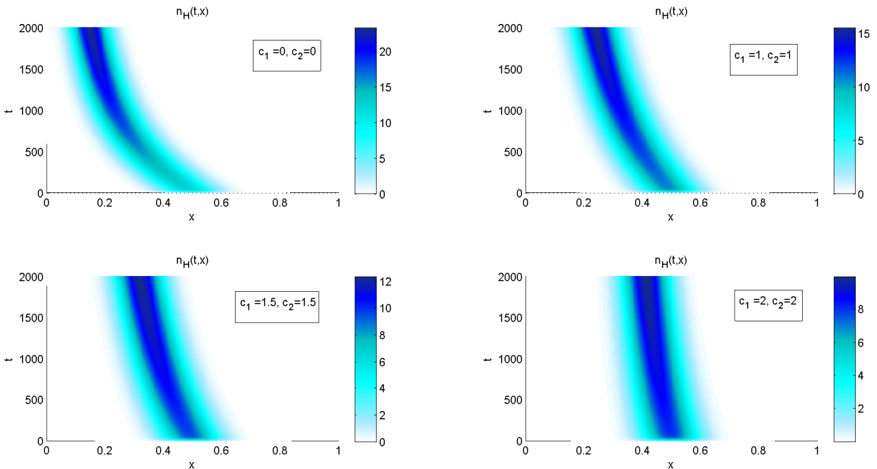
Figure 6.7: (Cytotoxic and cytostatic drugs) Dynamics of n_H(x,t) for c_1 = c_2 = 0 (top-left), c_1 = c_2 = 1 (top-right), c_1 = c_2 = 1.5 (bottom-left) and c_1 = c_2 = 2 (bottom-right). As long as parameters c_1 and c_2 increase, the maximum value of n_H(t = 2000, x) becomes smaller but about one half of the healthy cells is still alive at the end of computations.
