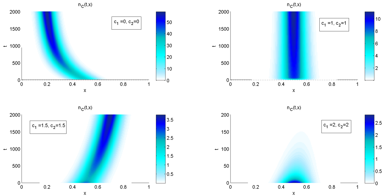
Figure 6.6: (Cytotoxic and cytostatic drugs) Dynamics of n_C(x, t) for c_1 = c_2 = 0 (top-left), c_1 = c_2 = 1 (top-right), c_1 = c_2 = 1.5 (bottom-left) and c_1 = c_2 = 2 (bottom-right). As long as parameters c_1 and c_2 increase, the maximum value of n_C(t = 2000, x) becomes smaller so that, under the choice c_1 = c_2 = 2 , function n_C(x, t) tends to zero across time.
