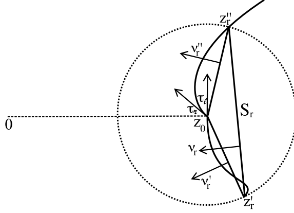
Fig. 7. The construction of \tilde{F} in the proof of Theorem 8.10.
