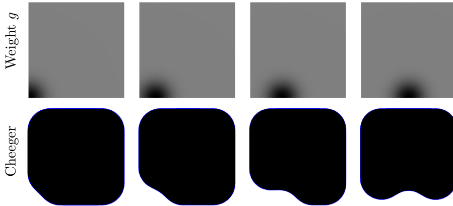
Figure 3: Cheeger sets in a 2D square with f = 1 and several non-constant weights g .
