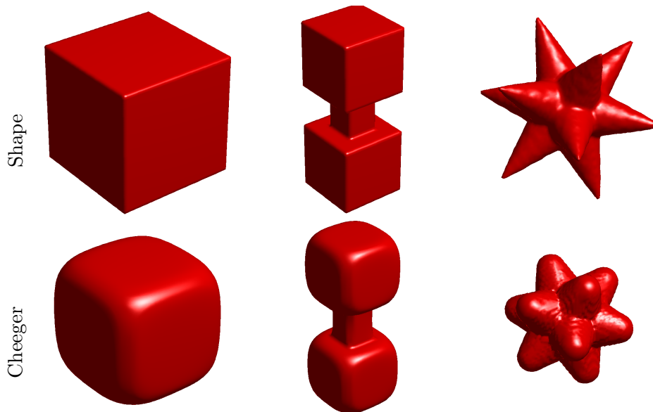
Figure 2: Cheeger sets in 3D with constant weights f = g = 1 .
