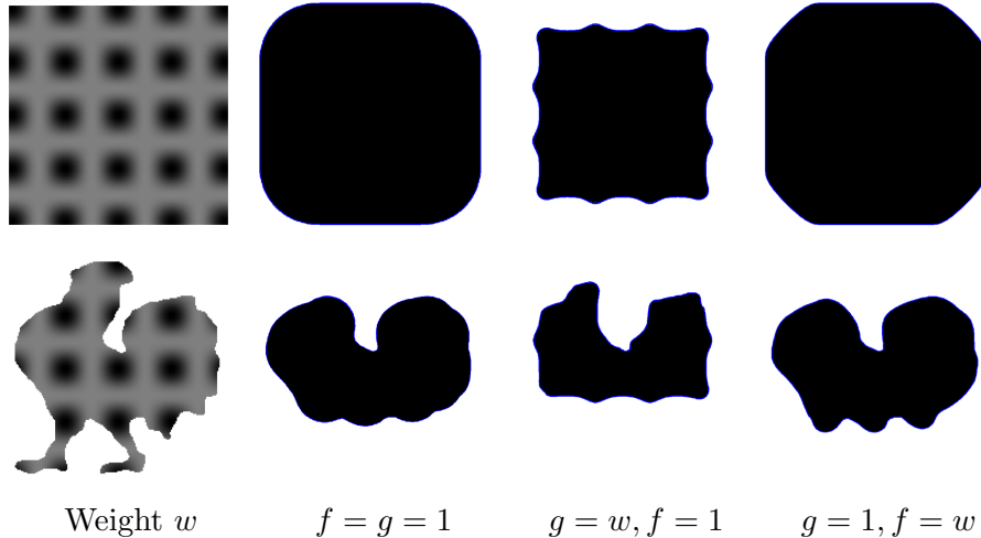
Figure 4: Comparison of the Cheeger with constant weights and with varying weights g or f .
