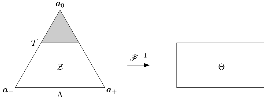
Figure 2: The homographic transformation from \mathcal{Z} onto \Theta
