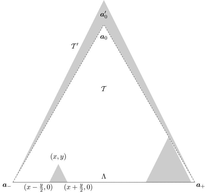
Figure 1: The lifting from \Lambda to triangles \mathcal{T} and \mathcal{T}'
