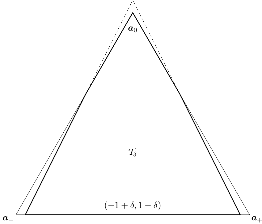
Figure 3: The polygon \mathcal{T}_\delta (with \delta = 0.08 )
