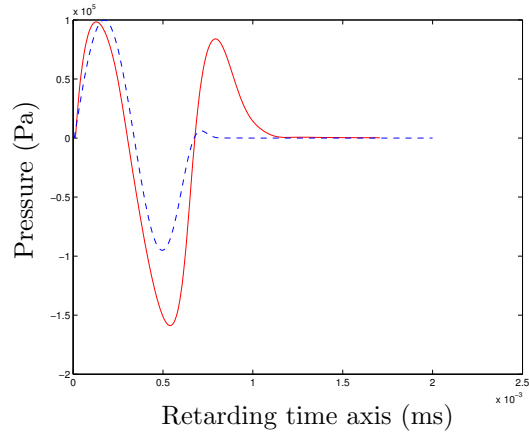
Figure 7: Representation of the solution of KZK equation (38) along the retarded axis \tau in the two different places of the propagation axis z with a square source 3 \text{ cm} \times 3 \text{ cm} . The dotted line corresponds to the signal source z = 0 and the solid line to the pressure at the distance z = 31.2 \text{ cm} . The parameters of simulation are the same as in figure 6.
